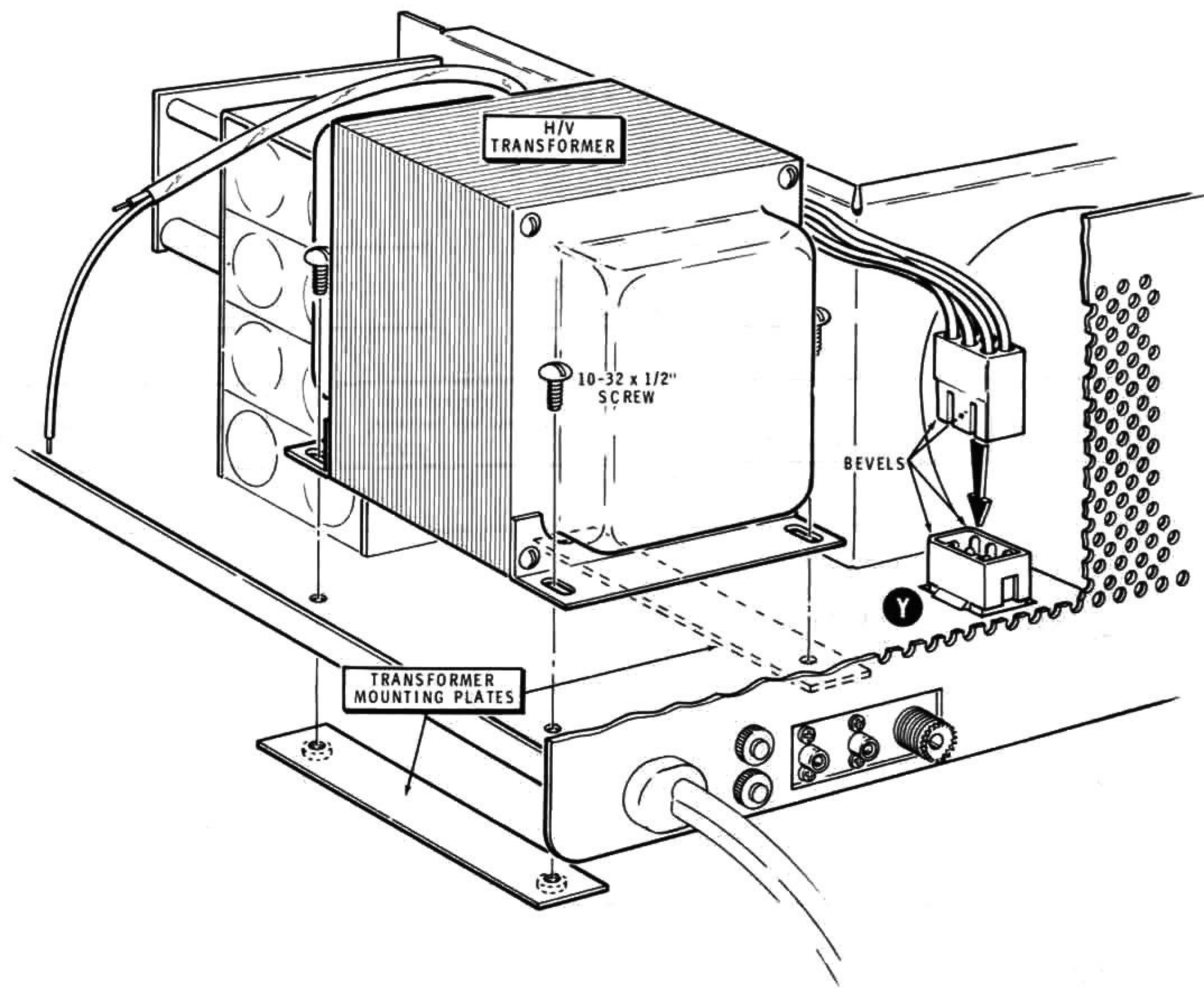
Detail 4-18A
